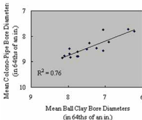
Figure 1. Scatter plot of Jamestown mean pipe bore diameters.
